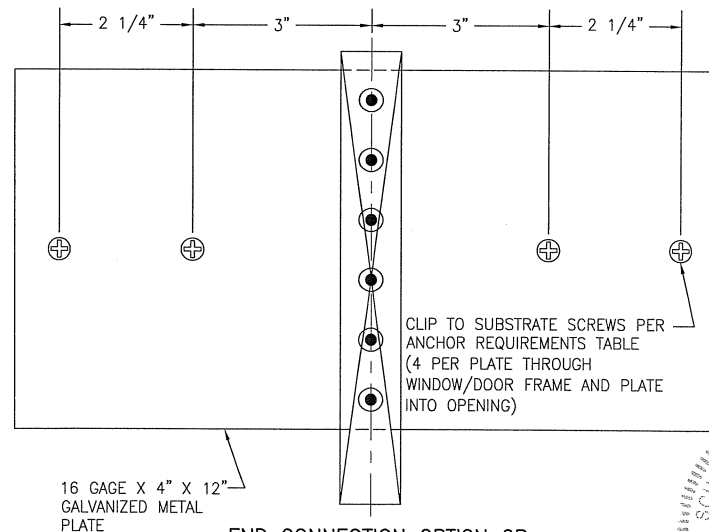
END CONNECTION OPTION 2B (SEE CONNECTION 2A FOR ATTACHMENT OF PLATE TO MULLION)
