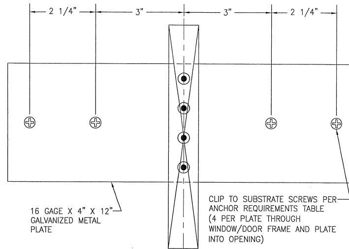
END CONNECTION OPTION 3B (SEE CONNECTION 3A FOR ATTACHMENT OF PLATE TO MULLION)
